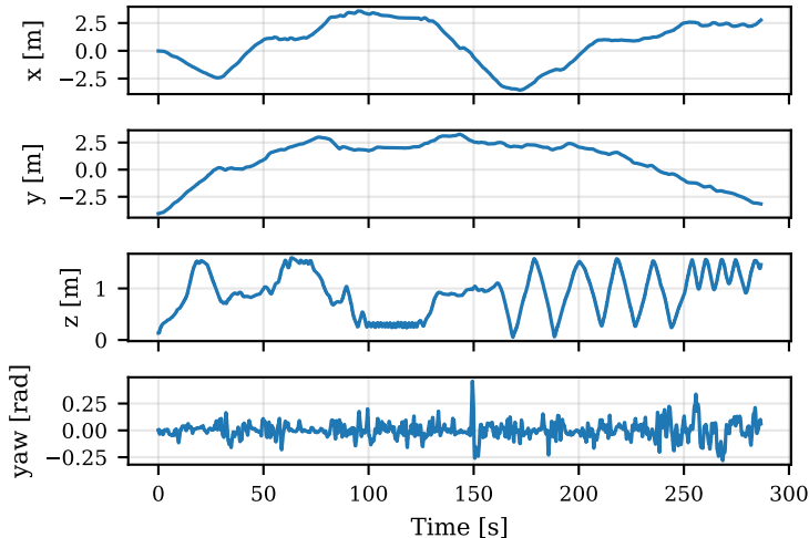
exp 9 - UAV 1 - Position
